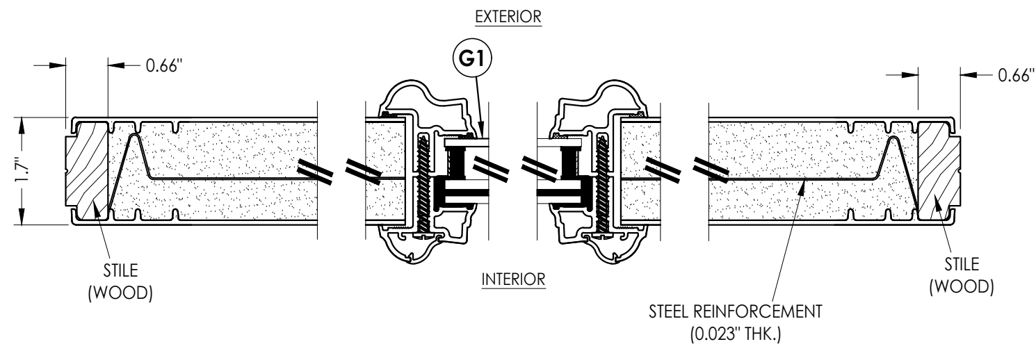
1 3 HORIZONTAL CROSS SECTION
